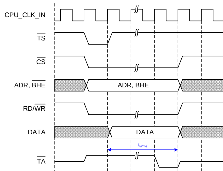
Figure 34: Write access (CS together with TS, Write DATA after CS, CS and TA on rising edge)
