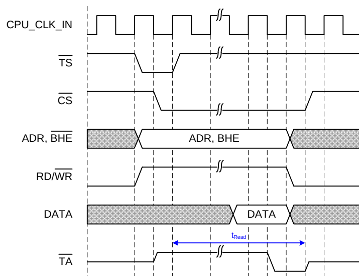
Figure 37: Read access (CS half a clock period after TS, CS and TA on falling edge)
