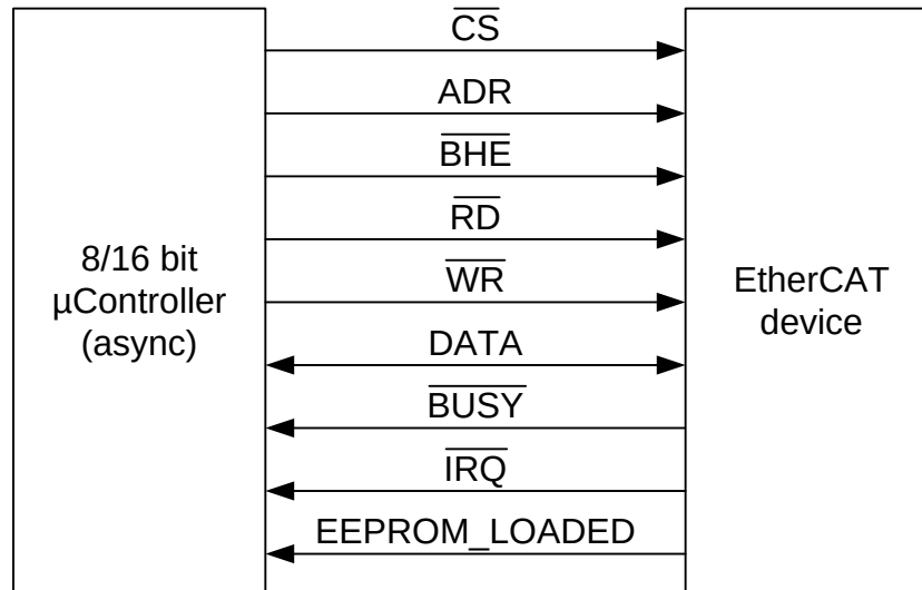
Figure 22: \mu Controller interconnection 3
