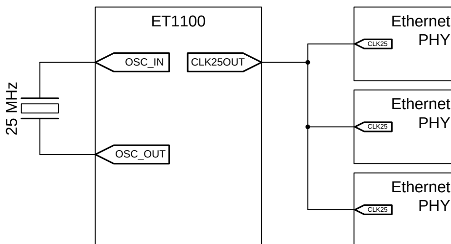
Figure 44: Quartz crystal Clock source for ET1100 and Ethernet PHYs
