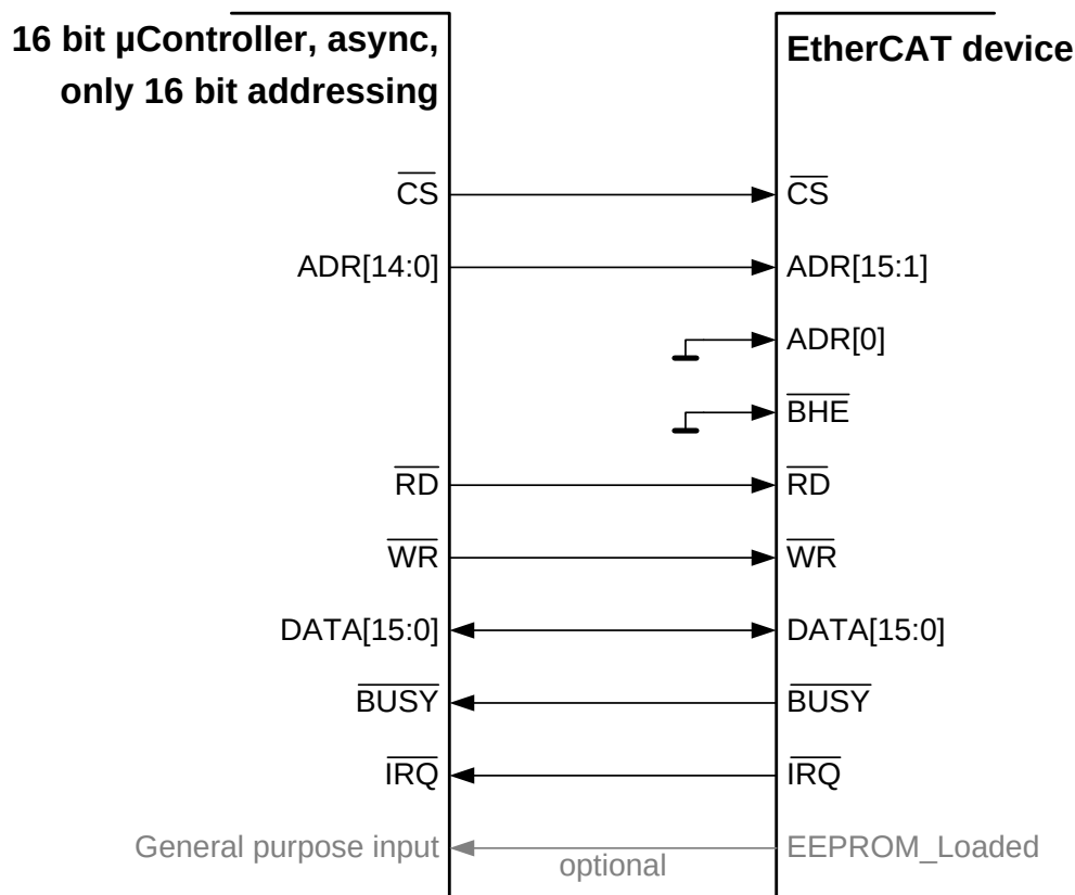
Figure 23: Connection with 16 bit \mu Controllers without byte addressing
