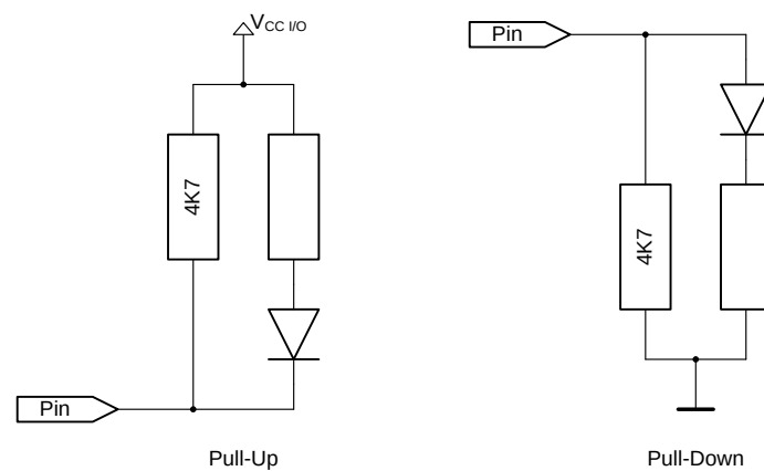
Figure 47: Dual purpose configuration input/LED output pins
