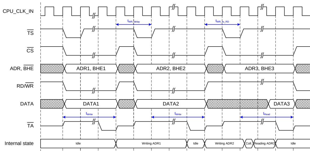
Figure 38: Sequence of two write accesses and a read access
