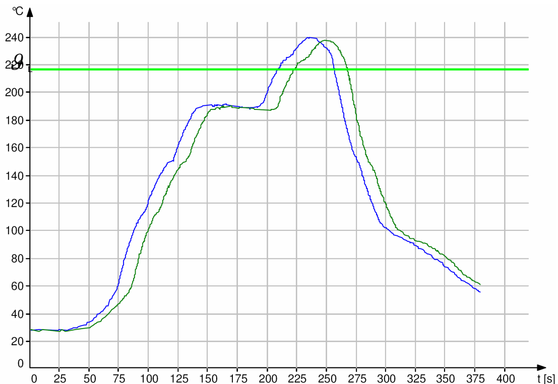
Figure 59: Example Soldering Profiles
