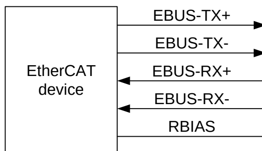
Figure 8: EBUS Interface Signals
