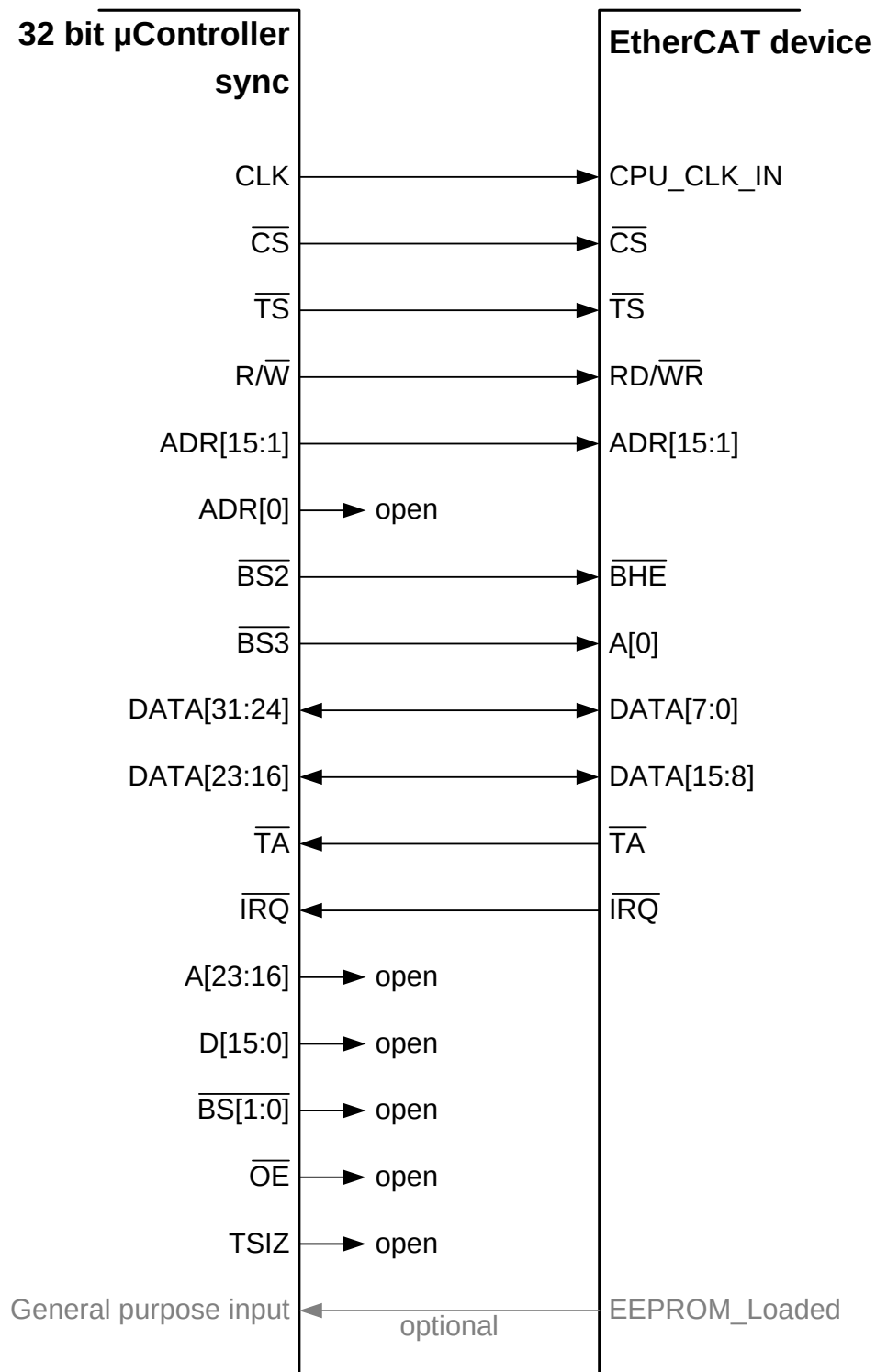
Figure 29: Synchronous 32 bit \mu Controller connection using Byte Select
