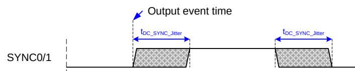
Figure 41: SyncSignal timing
