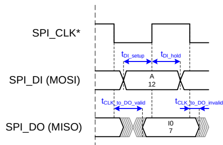
Figure 17: Basic SPI_DI/SPI_DO timing (*refer to timing diagram for relevant edges of SPI_CLK)
