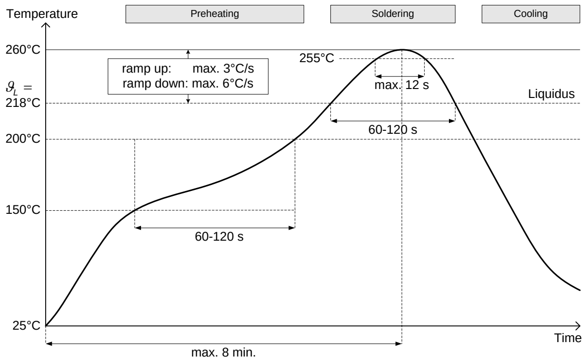
Figure 58: Maximum Soldering Profile
