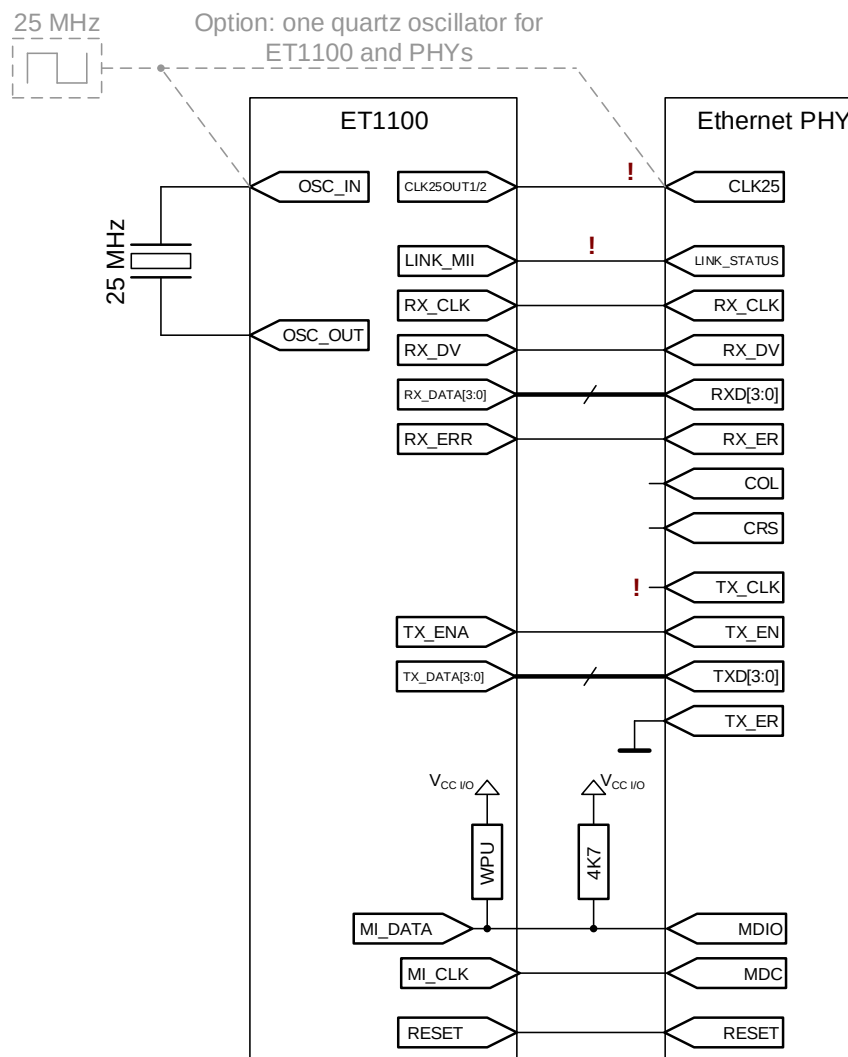
Figure 48: PHY Connection
