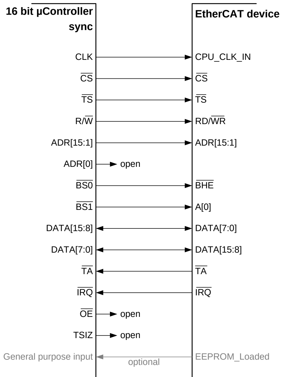
Figure 30: Synchronous 16 bit \mu Controller connection using Byte Select
