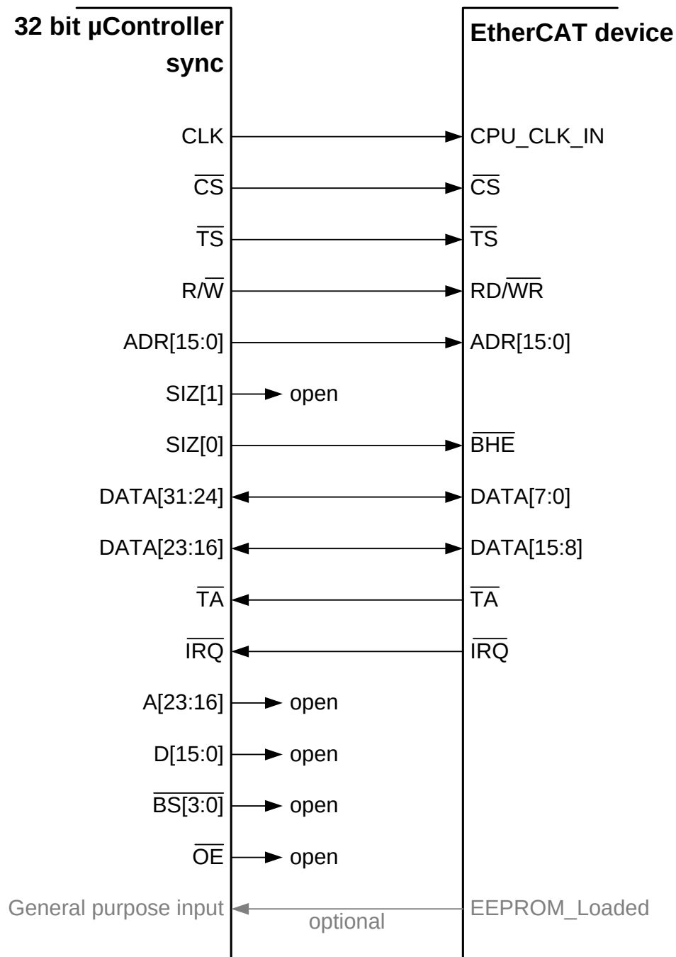
Figure 31: Synchronous 32 bit \mu Controller connection using Transfer Size
