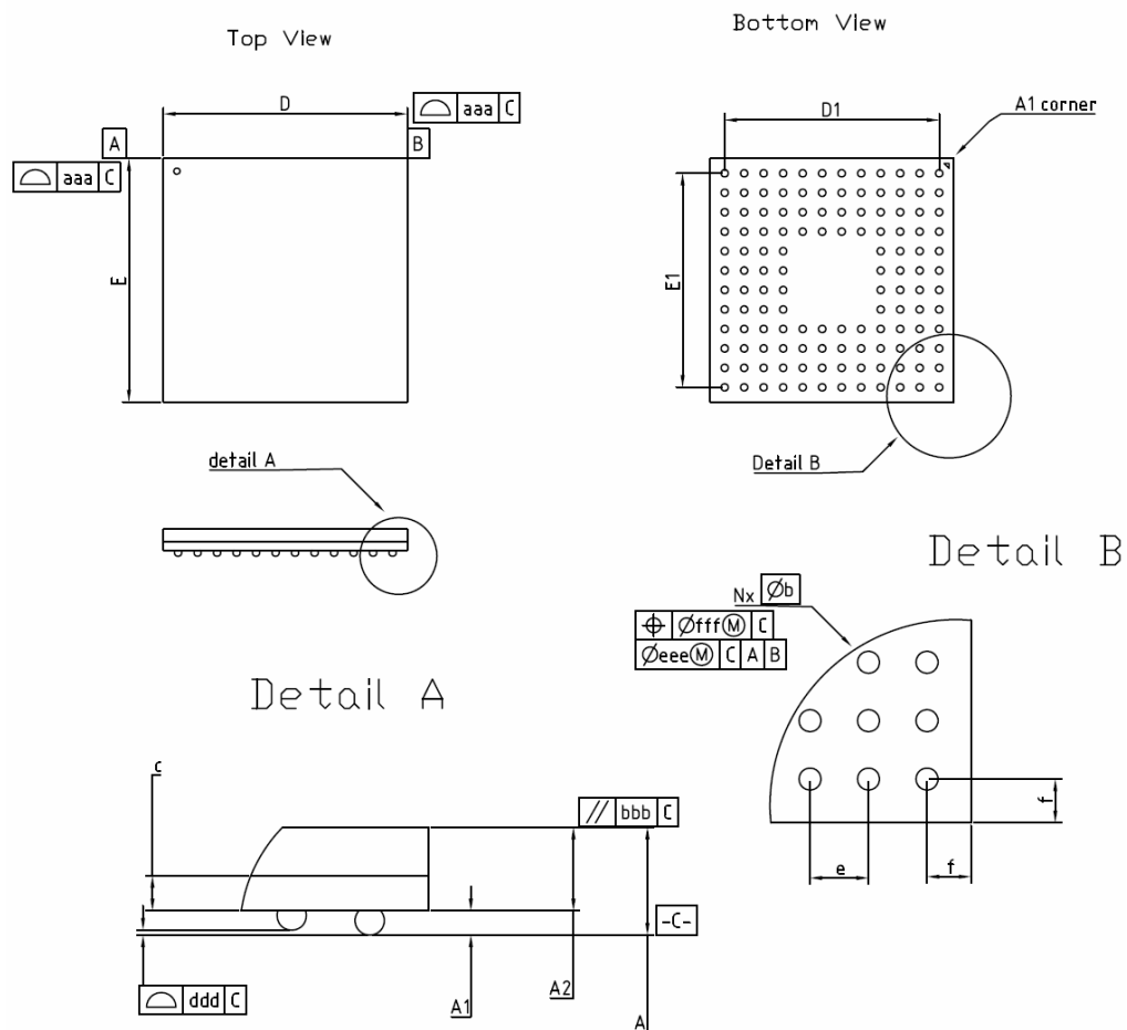
Figure 54: Package Outline
