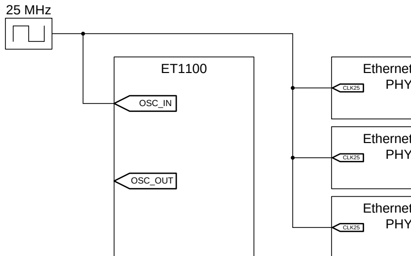
Figure 45: Oscillator clock source for ET1100 and Ethernet PHYs
