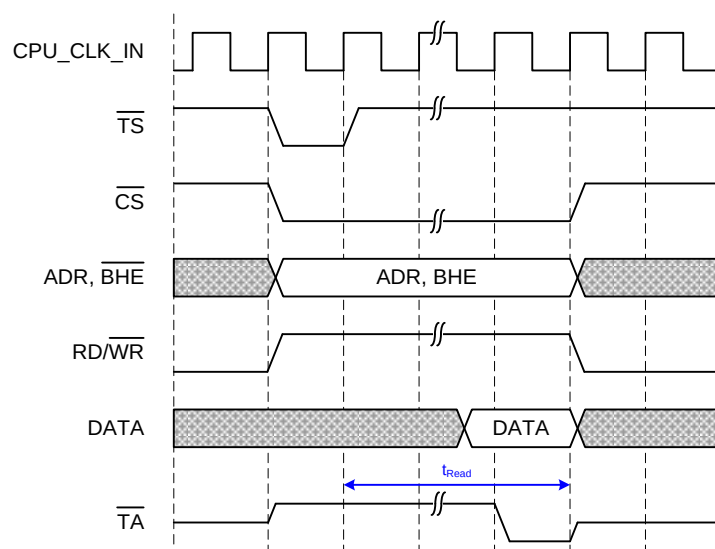
Figure 36: Read access (CS together with TS, CS and TA on rising edge)
