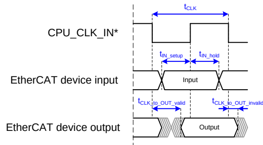
Figure 32: Basic synchronous \mu Controller interface timing (*refer to timing diagram for relevant CPU_CLK_IN edges)
