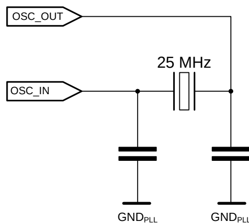
Figure 43: Quartz crystal connection
