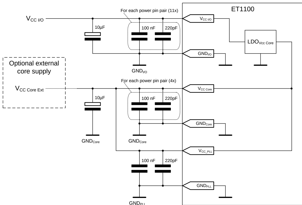
Figure 46: ET1100 power supply
