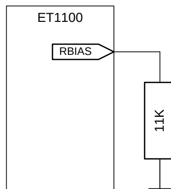
Figure 50: LVDS load resistor
