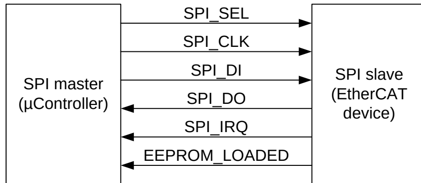
Figure 16: SPI master and slave interconnection
