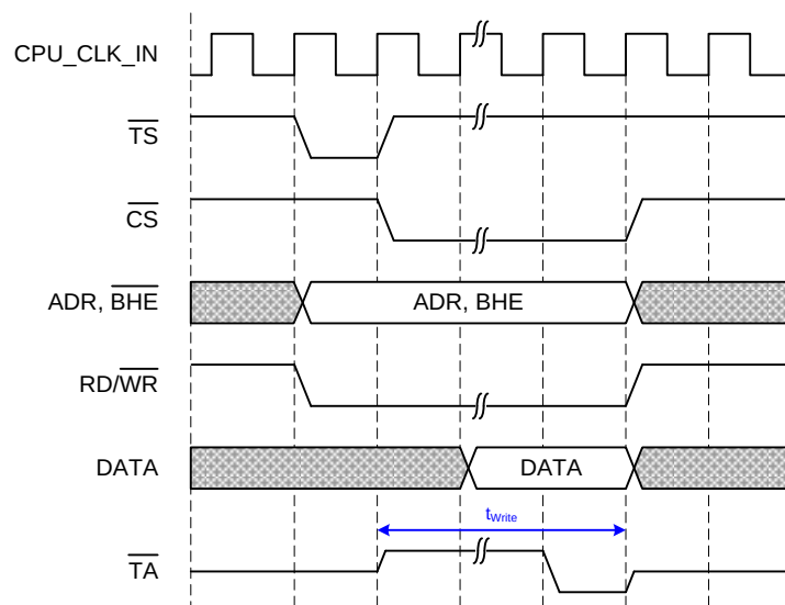
Figure 35: Write access (CS after TS, Write DATA after CS, CS and TA on rising edge)
