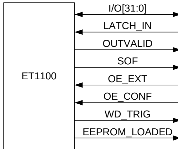
Figure 9: ET1100 Digital I/O signals
