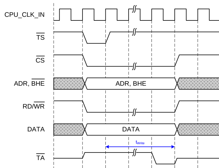
Figure 33: Write access (CS together with TS, Write DATA together with CS, CS and TA on rising edge)
