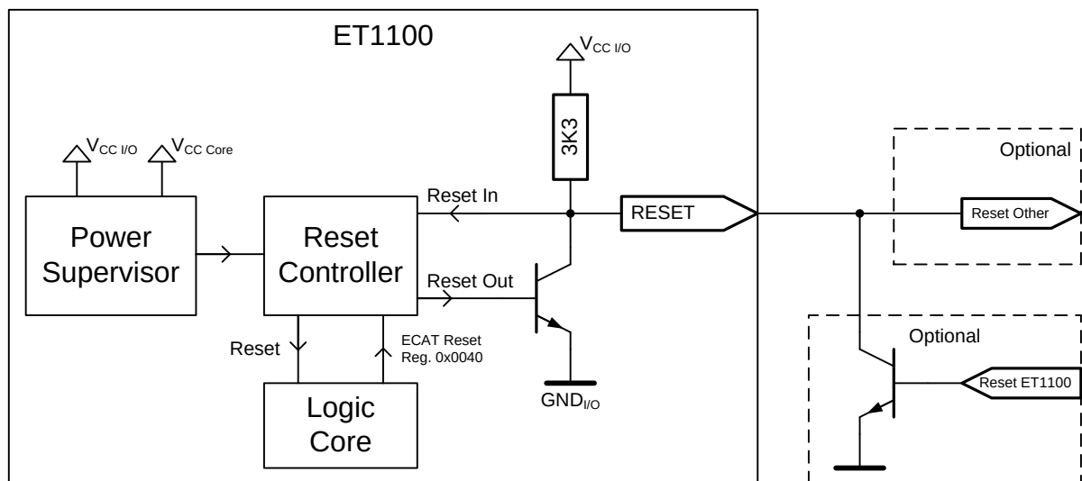
Figure 51: Reset Logic
