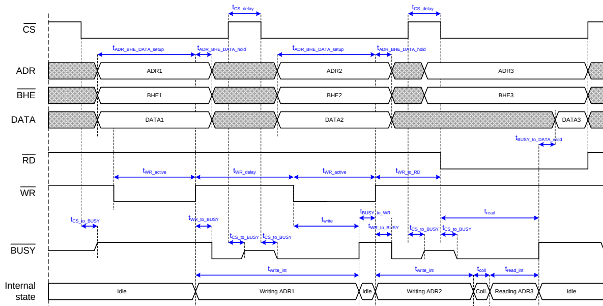
Figure 27: Sequence of two write accesses and a read access
