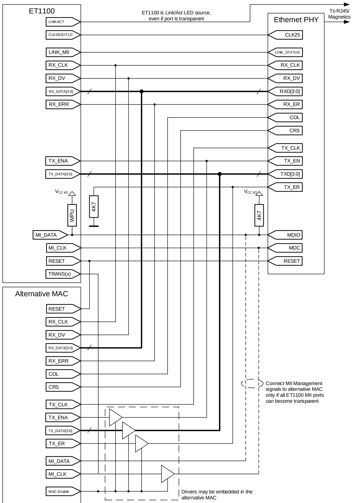
Figure 52: Transparent Mode
