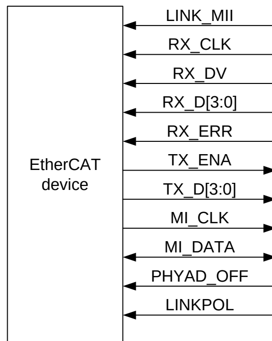
Figure 5: MII Interface signals
