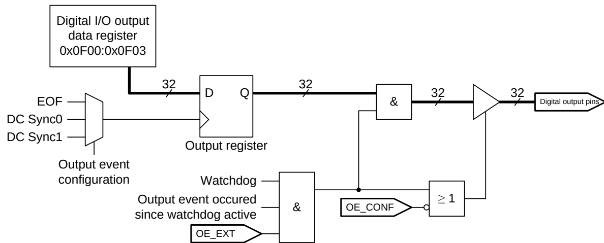
Figure 10: Digital Output Principle Schematic
