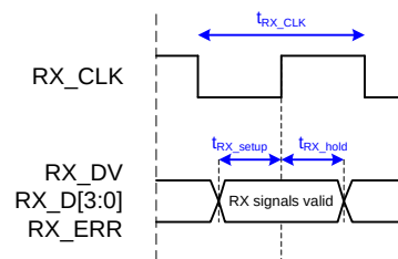
Figure 7: MII timing RX signals
