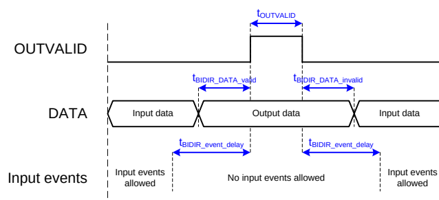
Figure 15: Bidirectional Mode timing
