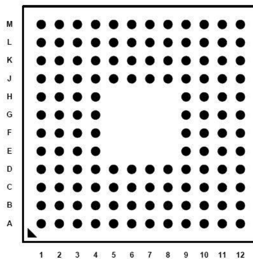
Figure 55: TFBGA 128 Pin Layout
