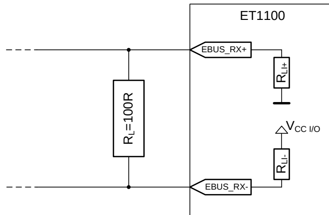
Figure 49: LVDS termination
