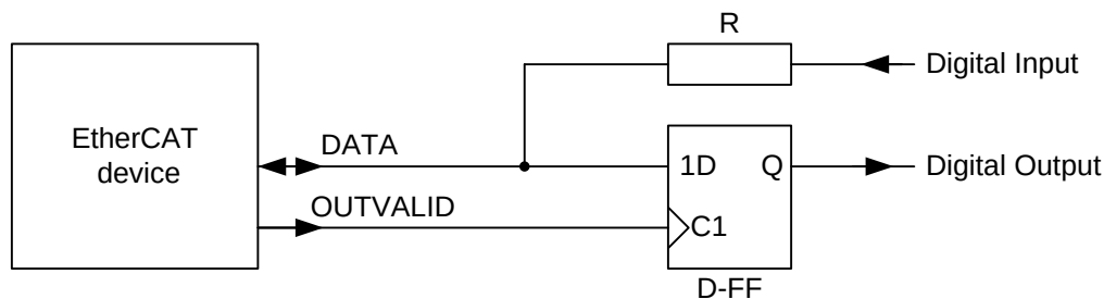
Figure 11: Bidirectional mode: Input/Output connection (R=4.7 kΩ recommended)
